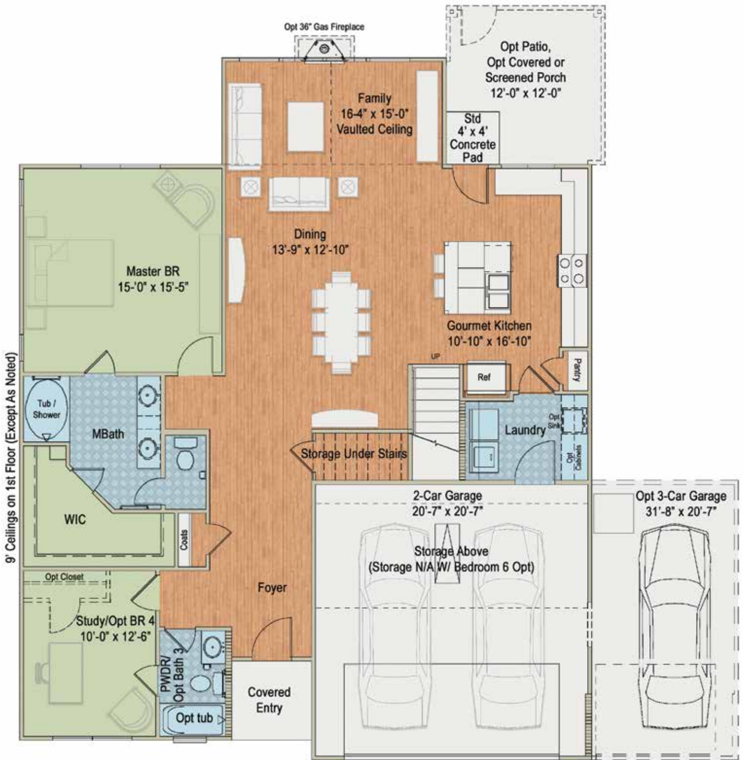
BASE FLOOR PLAN ~2,125 SQUARE FEET
